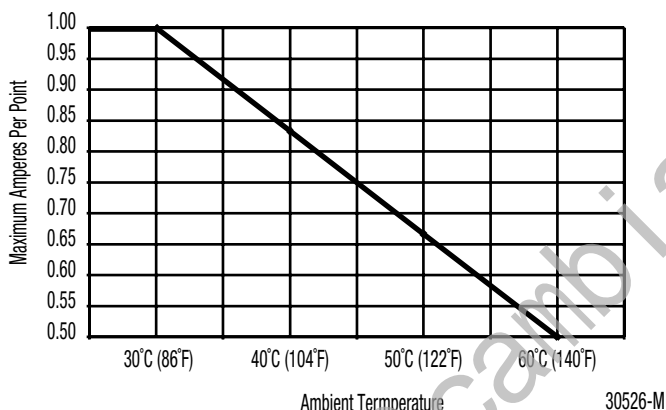
1769-0B32 Maximum Amperes per Point vs. Temperature
